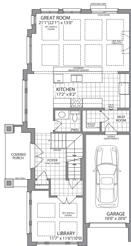
MAIN LEVEL - ELEV. B
