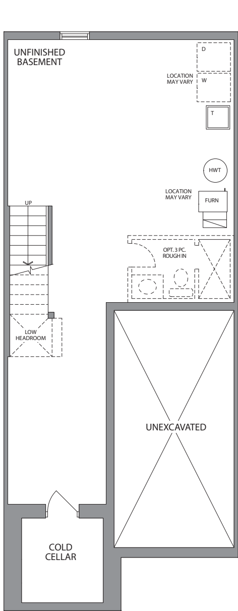
LOWER LEVEL ELEV. A
