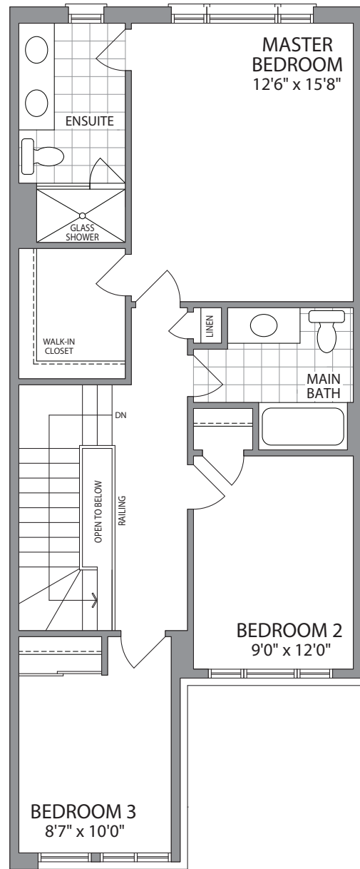
UPPER LEVEL - ELEV. B
