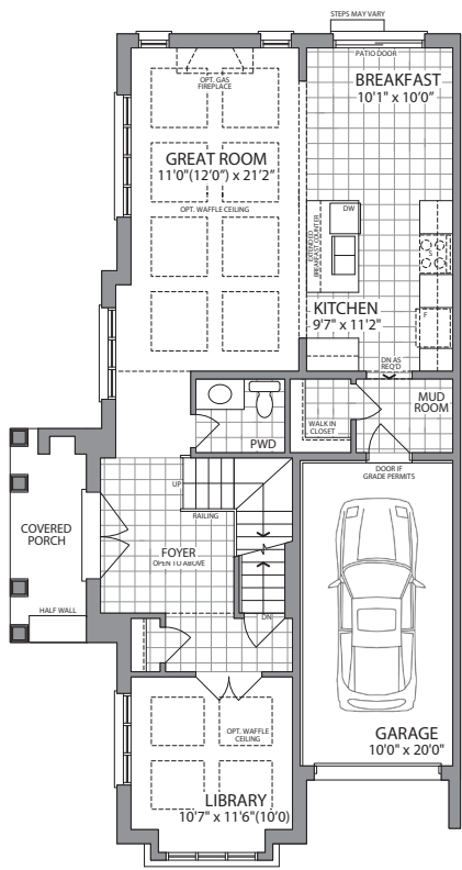
ALT. MAIN LEVEL - ELEV. A
