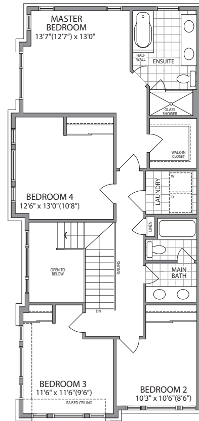
UPPER LEVEL - ELEV. B
