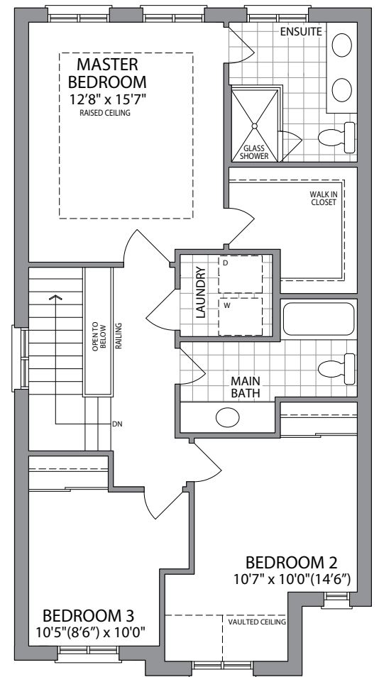
UPPER LEVEL - ELEV. B
