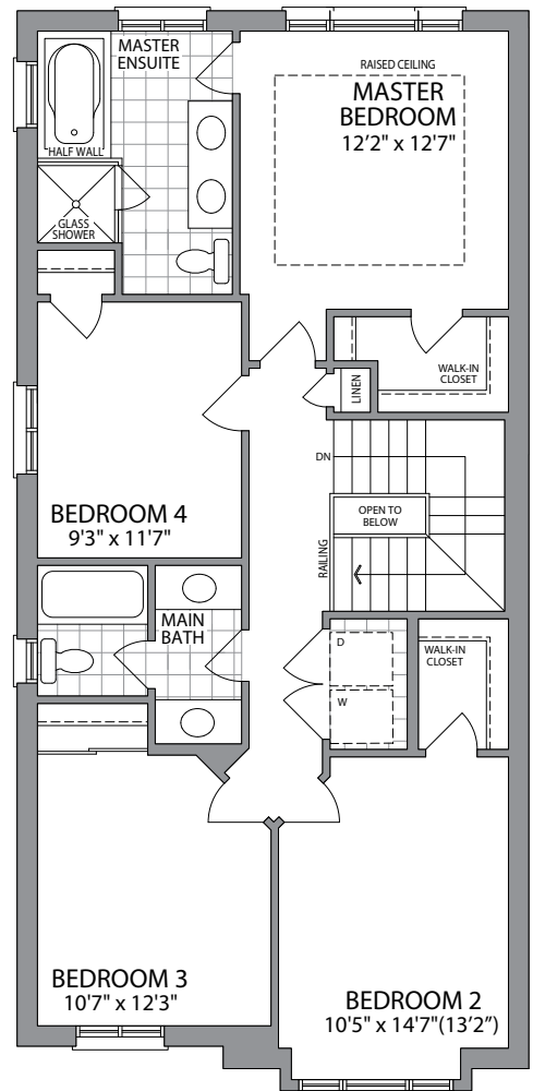
UPPER LEVEL - ELEV. B
