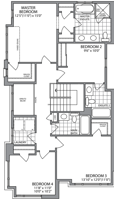
UPPER LEVEL - ELEV. C
