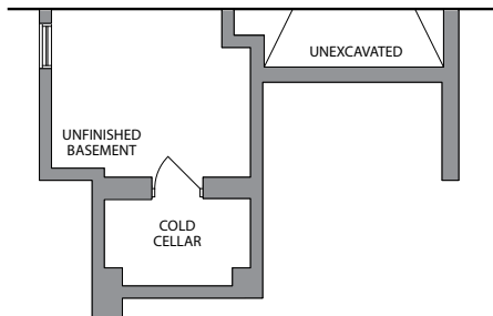
PART. LOWER LEVEL ELEV. C
