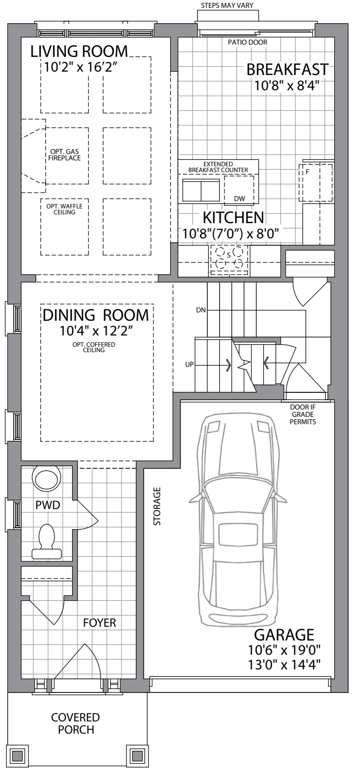
MAIN LEVEL - ELEV. A
