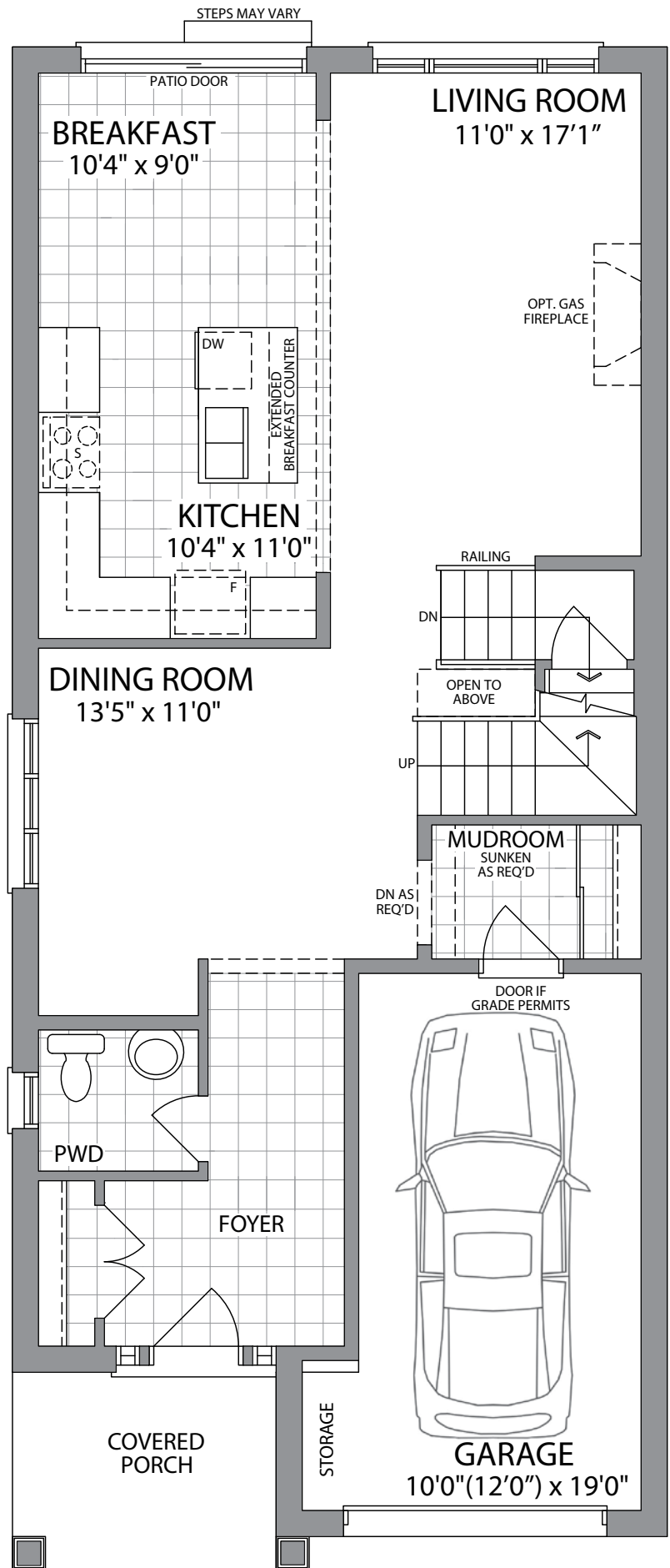
MAIN LEVEL - ELEV. A
