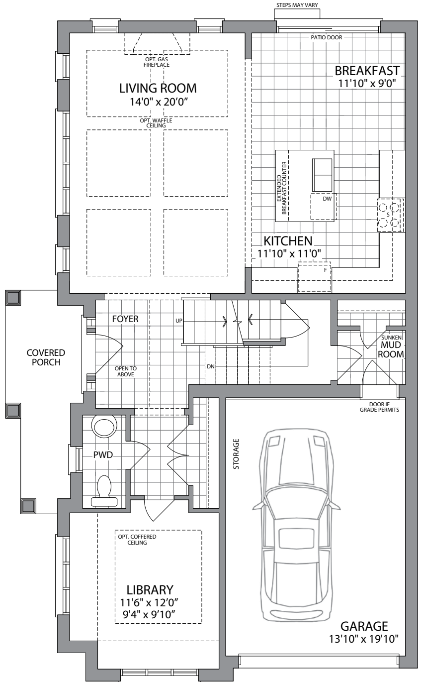
MAIN LEVEL - ELEV. A
