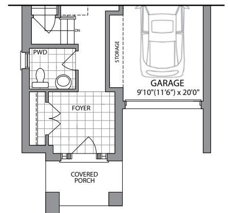
PART. MAIN LEVEL ELEV. C
