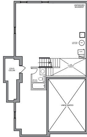
LOWER LEVEL ELEV. A
