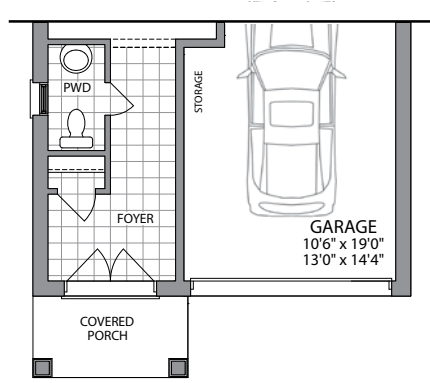
PART. MAIN LEVEL ELEV. B
